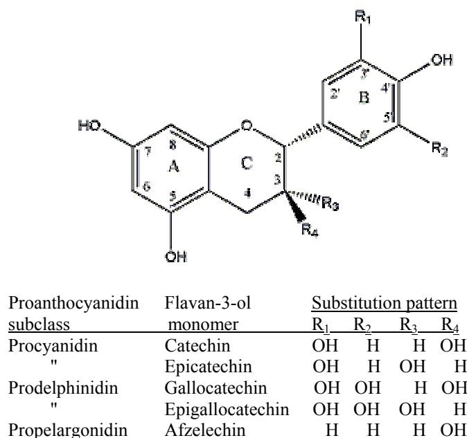
Figure 1. Structure of common flavan-3-ols and substitution patterns found in proanthocyanidins extracted from foods.
