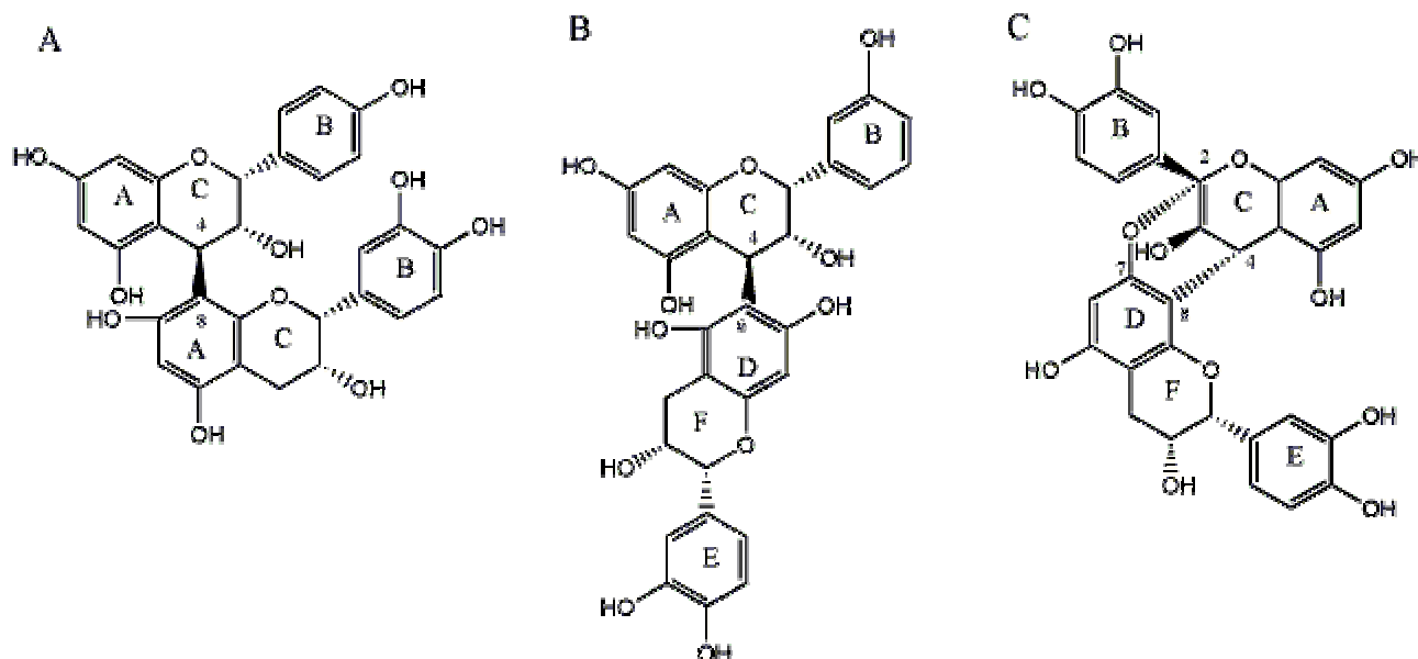
Figure 2. Common interflavan linkages found in proanthocyanidins extracted from foods. A) B type 4→8 linkage [Epicatechin-(4$→$8)-epicatechin], B) B type 4→6 linkage [Epicatechin-(4$→$6)-epicatechin], C) A type linkage [Epicatechin-(2$→$7, 4$→$8)-epicatechin]. From Porter, 1994.
